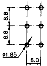
FOR "2" & "3" PC MOUNTING
